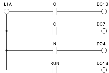
Contacts off: Existing Open & Close relays (if both used) and Nudging
