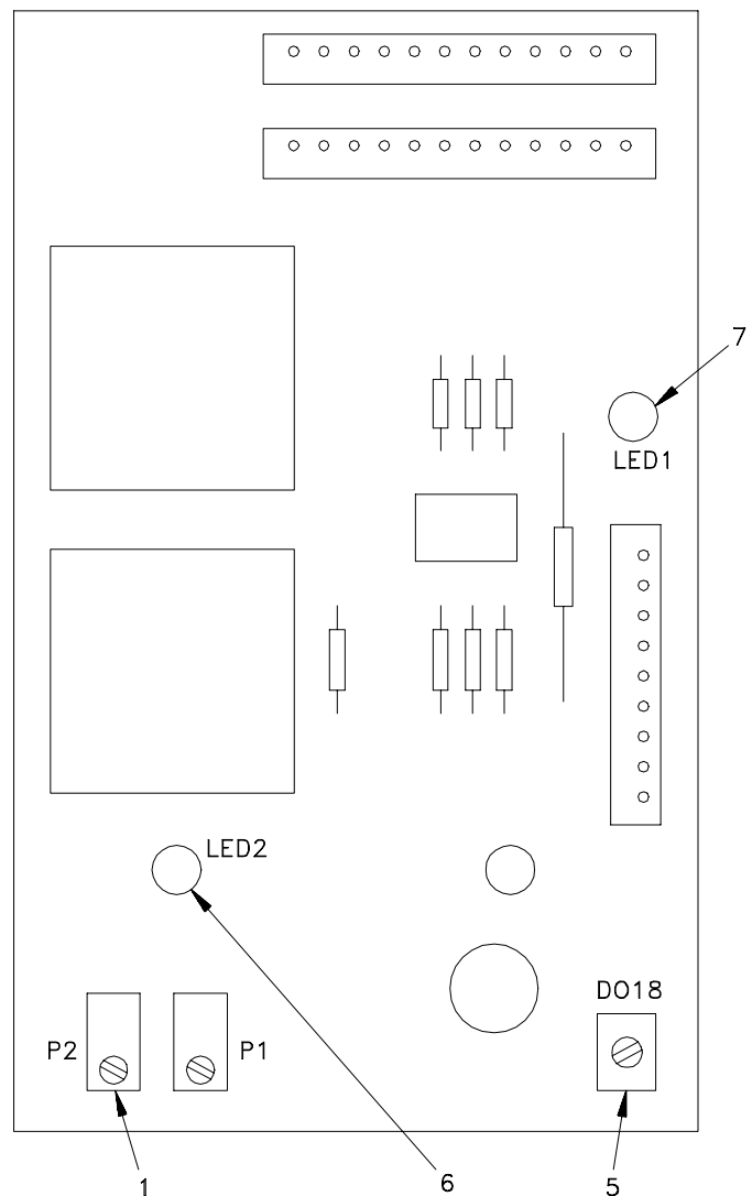
Auxiliary locking board
